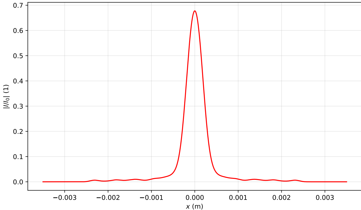
Intensity profile I(x, y = 0, z = 3.503)/I_0 , \text{Pin}=3.0\text{Pcr} , artificial time
